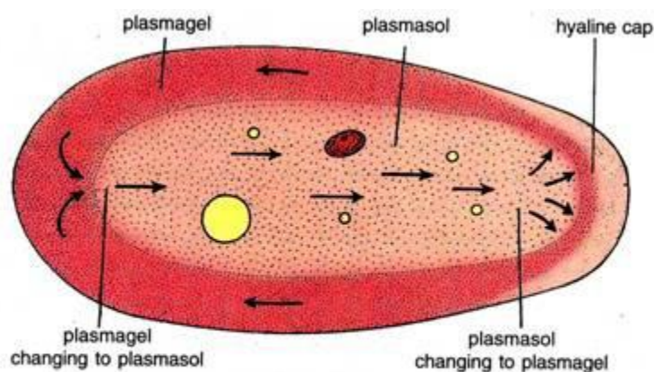
Fig. 14.10. Diagram illustrating the amoeboid movement on the basis of hydraulic pressure theory of Rinaldi and Jahn (1963).
